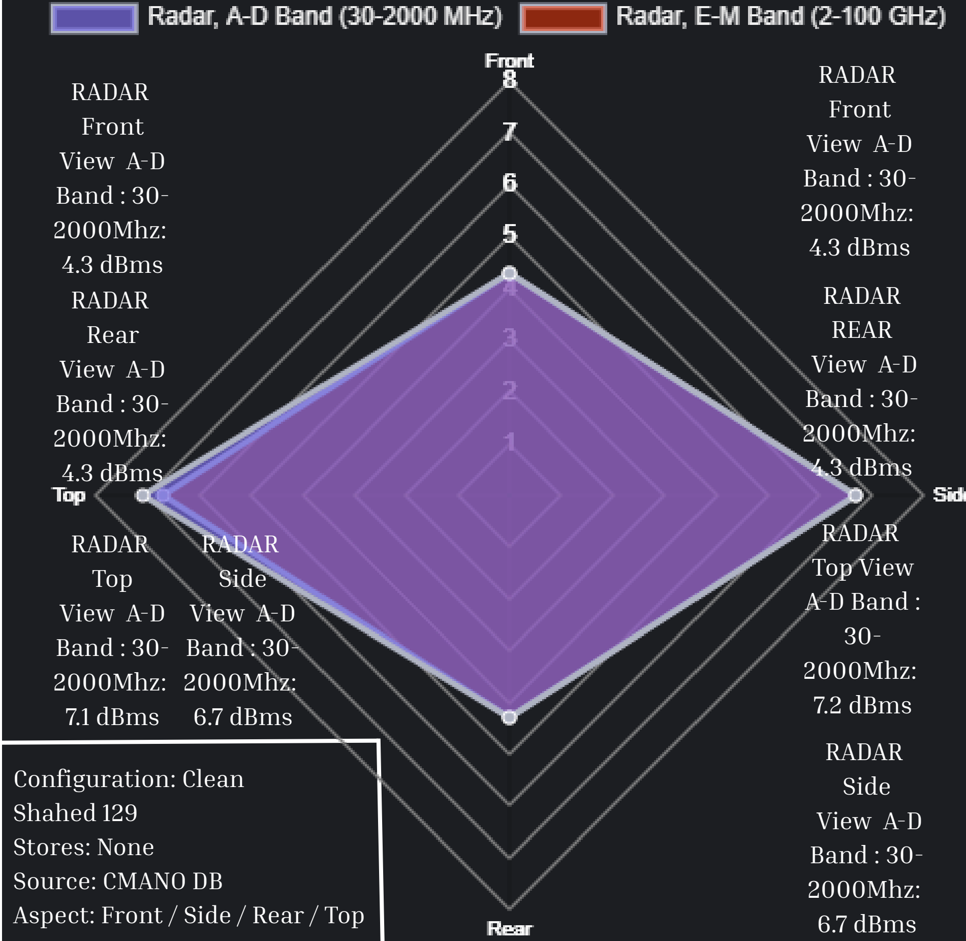
Signatures (dBsm)
